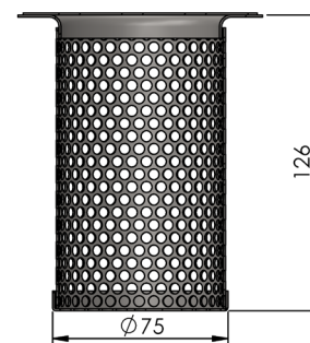
SECTION
